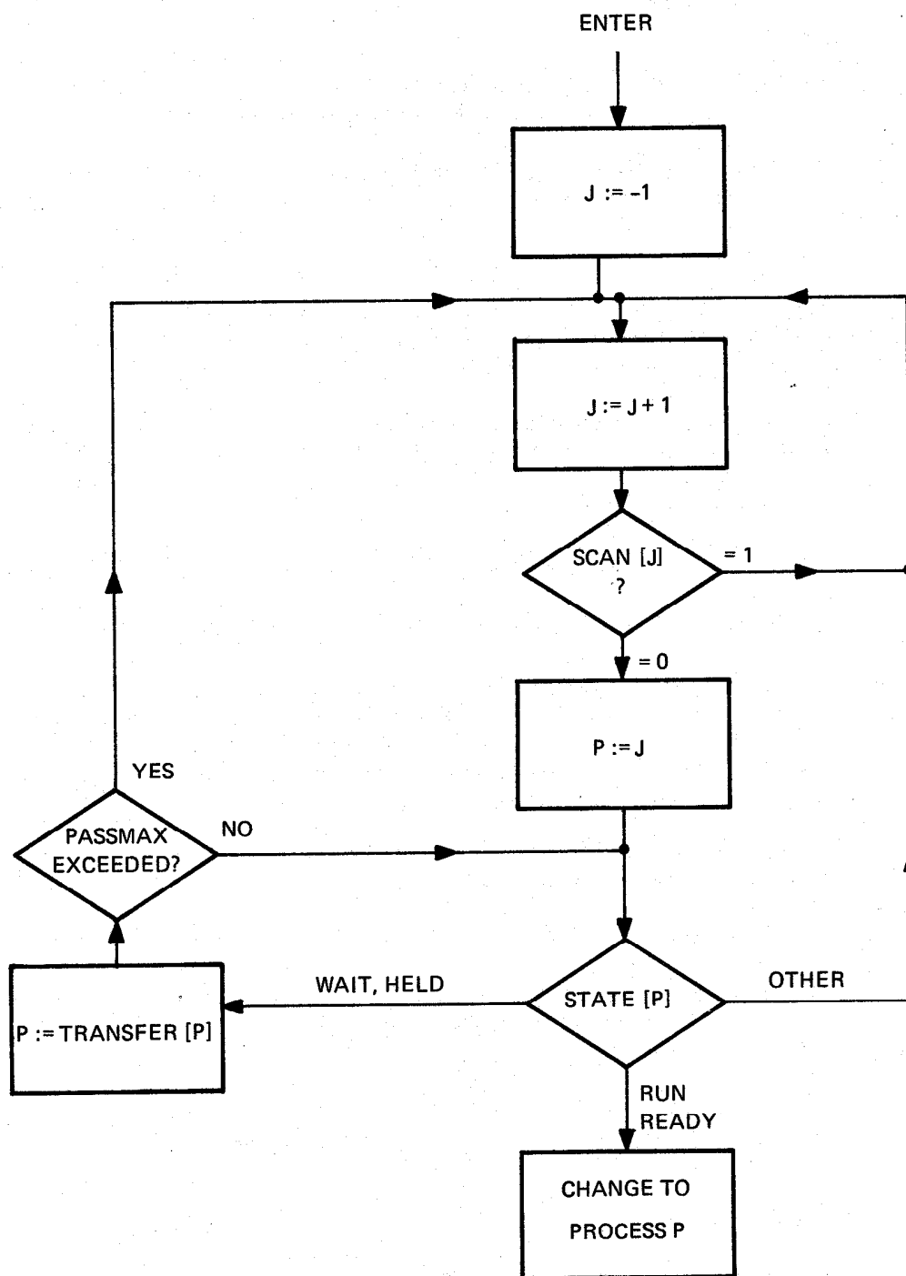
Figure 17: PROCESS SELECTOR OPERATION
