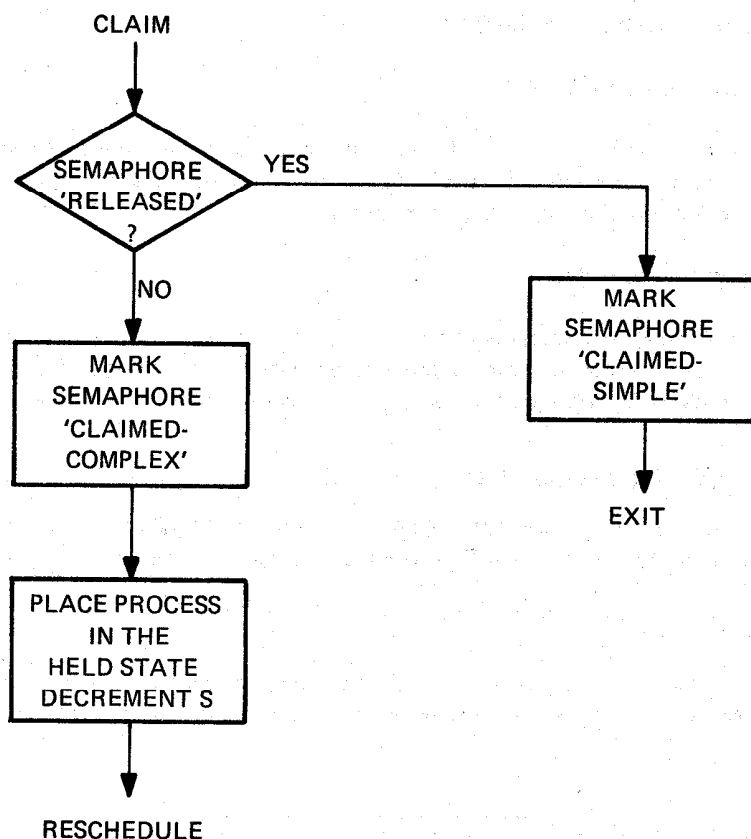
Figure 13: SEMAPHORE CLAIM
