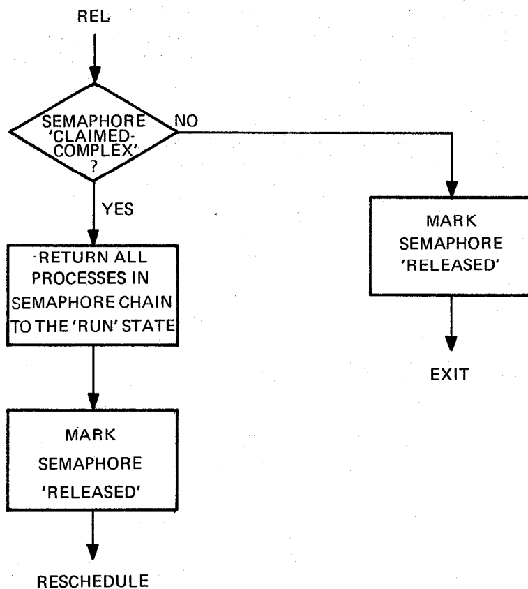
Figure 14: SEMAPHORE RELEASE
