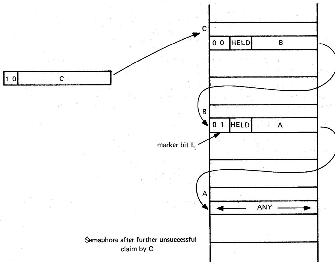
Figure 15: SEMAPHORE CHAINS
