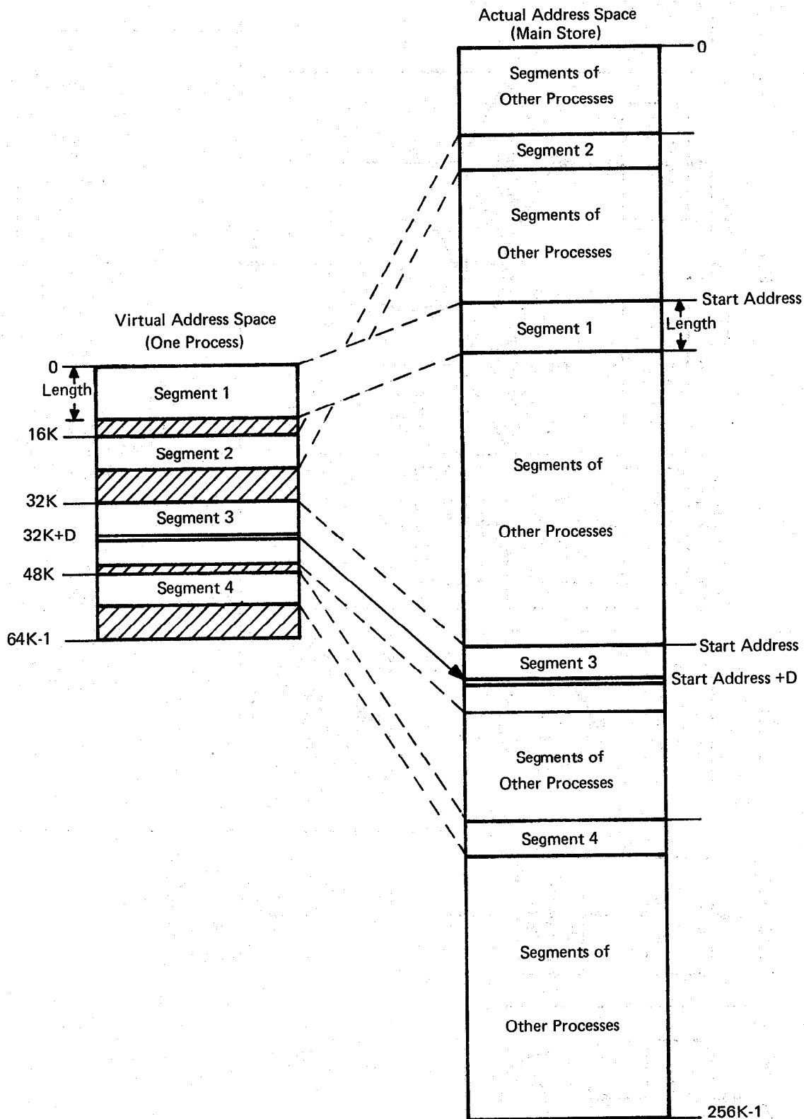
Figure 2: AN EXAMPLE OF VIRTUAL TO ACTUAL ADDRESS RELATIONSHIP
