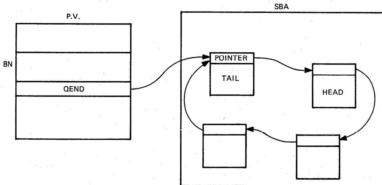
Figure 8: INCOMING MESSAGE QUEUE (PROCESS N)
