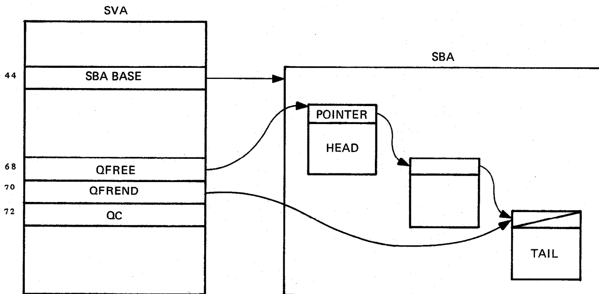
Figure 7: THE FREEQUEUE
