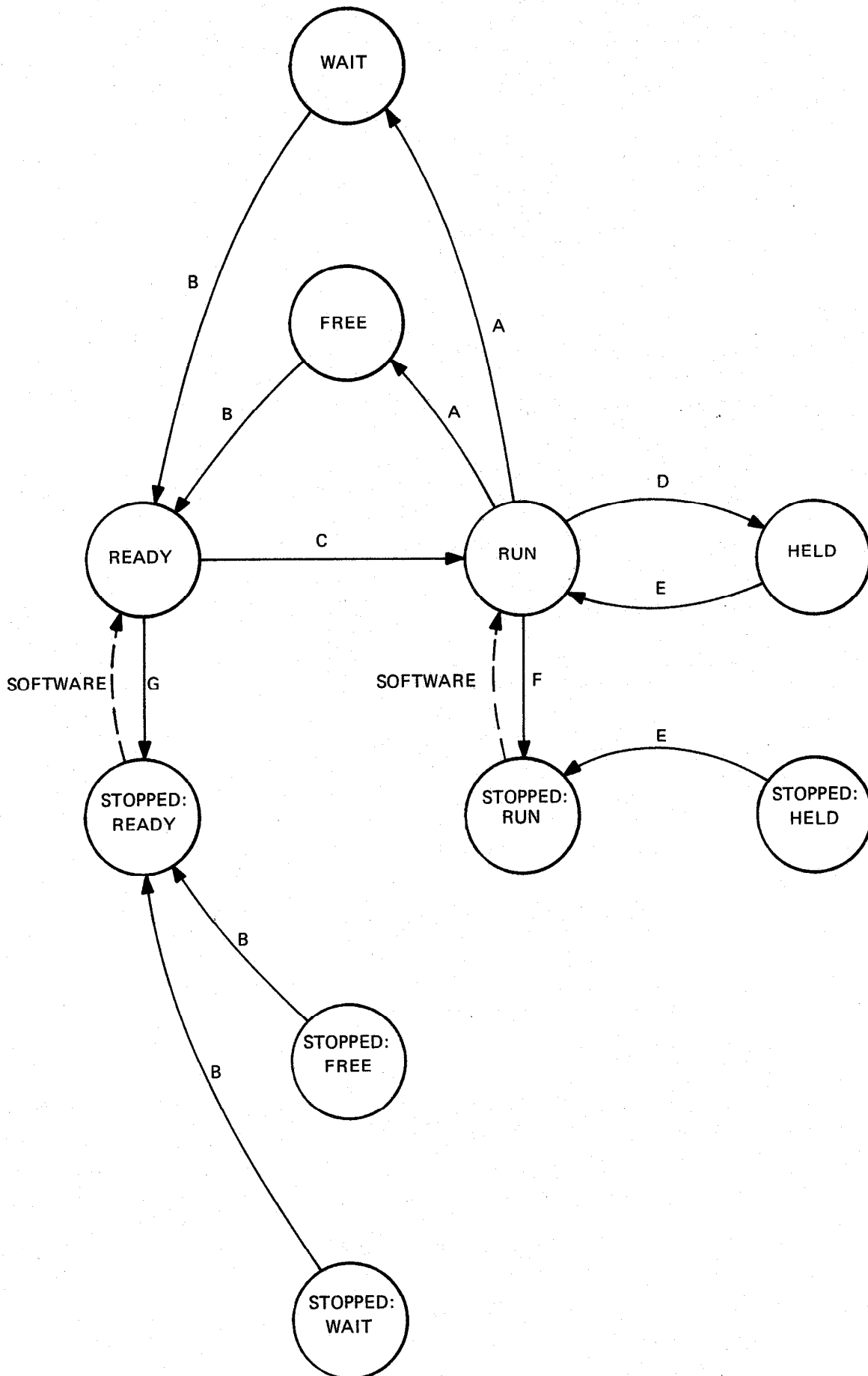
Figure 16: STATE TRANSITIONS
