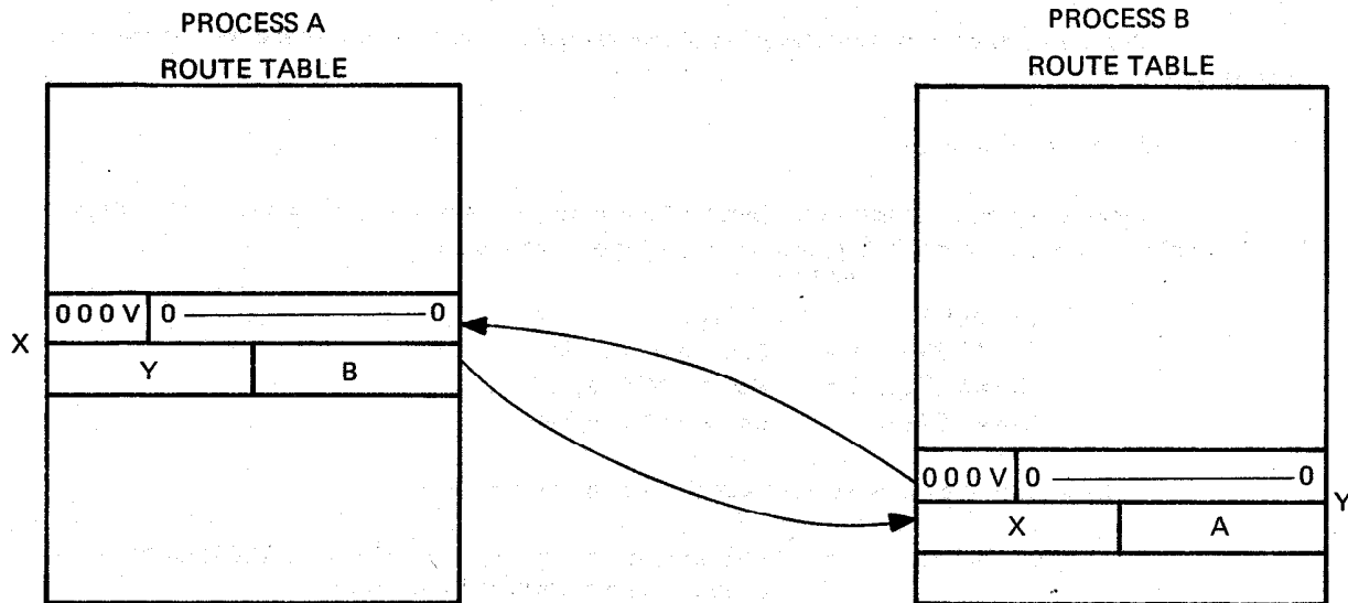
Figure 6: ROUTE PAIRS
